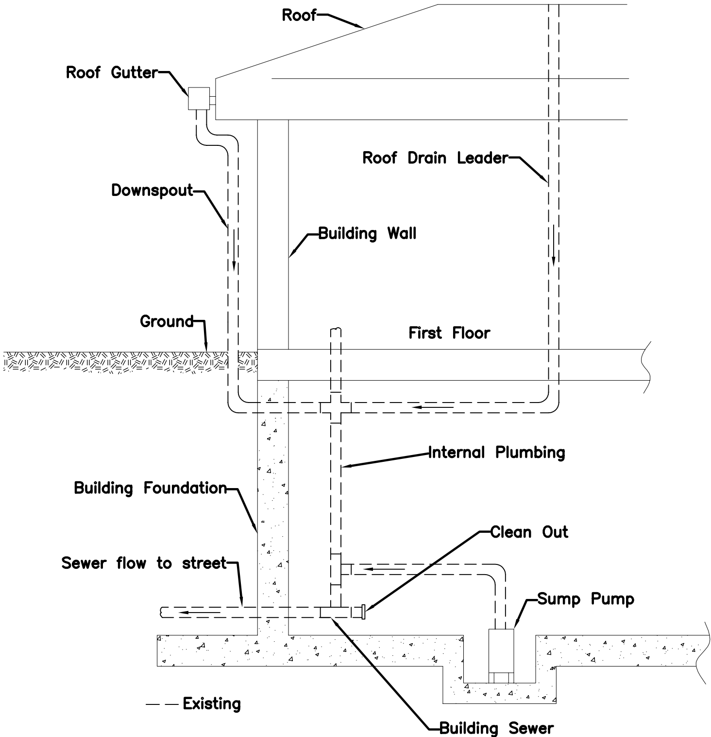
Typical Building Sewer Illustration
