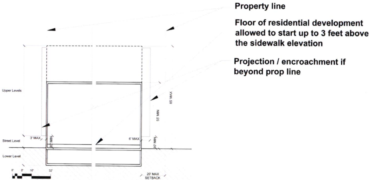
Vertical Dimension Standard Section A-A
